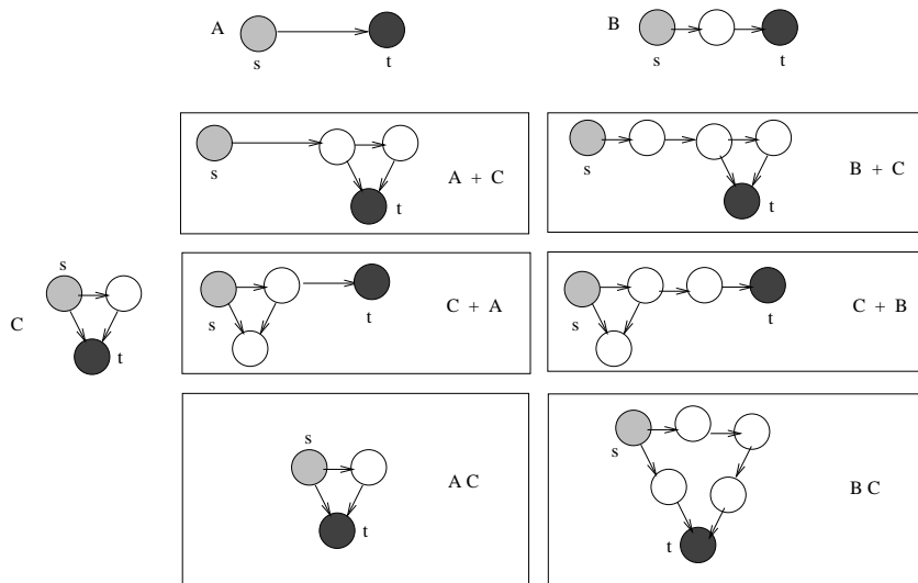
Figure 12: Strong order violations: (i). A+C \not\preceq B+C , (ii). C+A \not\preceq C+B , and (iii). AC \not\preceq BC .
